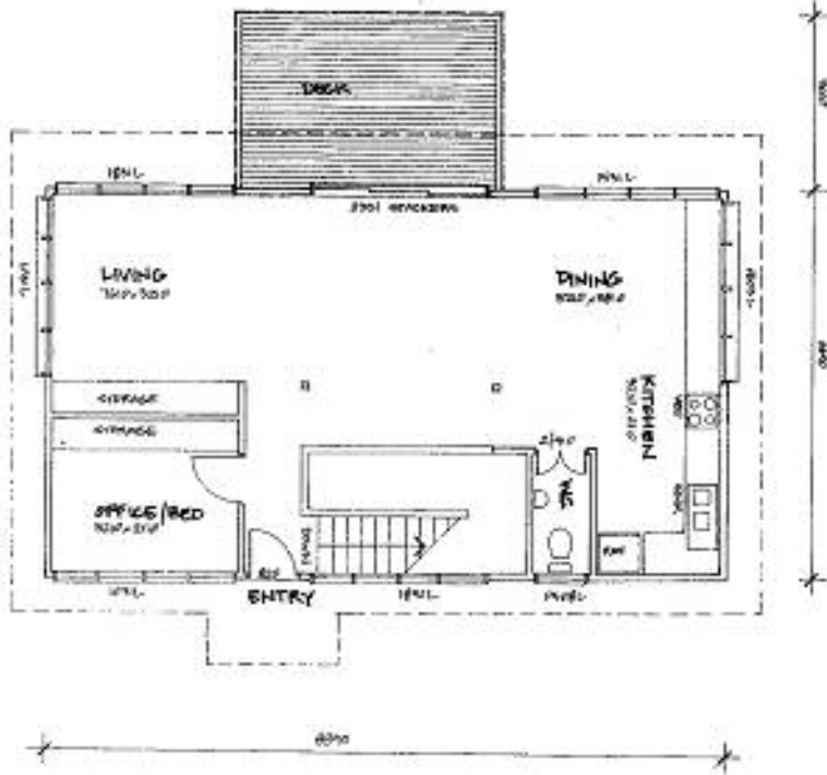
1 UPPER FLOOR
